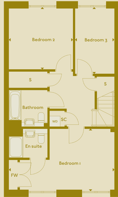
Third Floor
